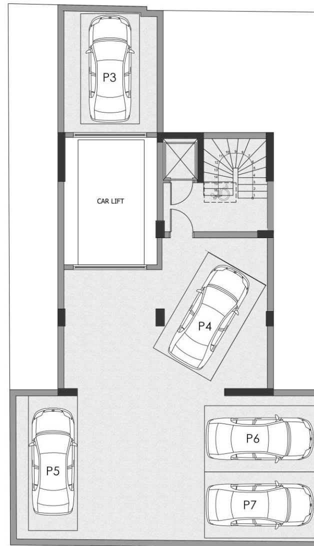
DELFFON Str BASEMENT
